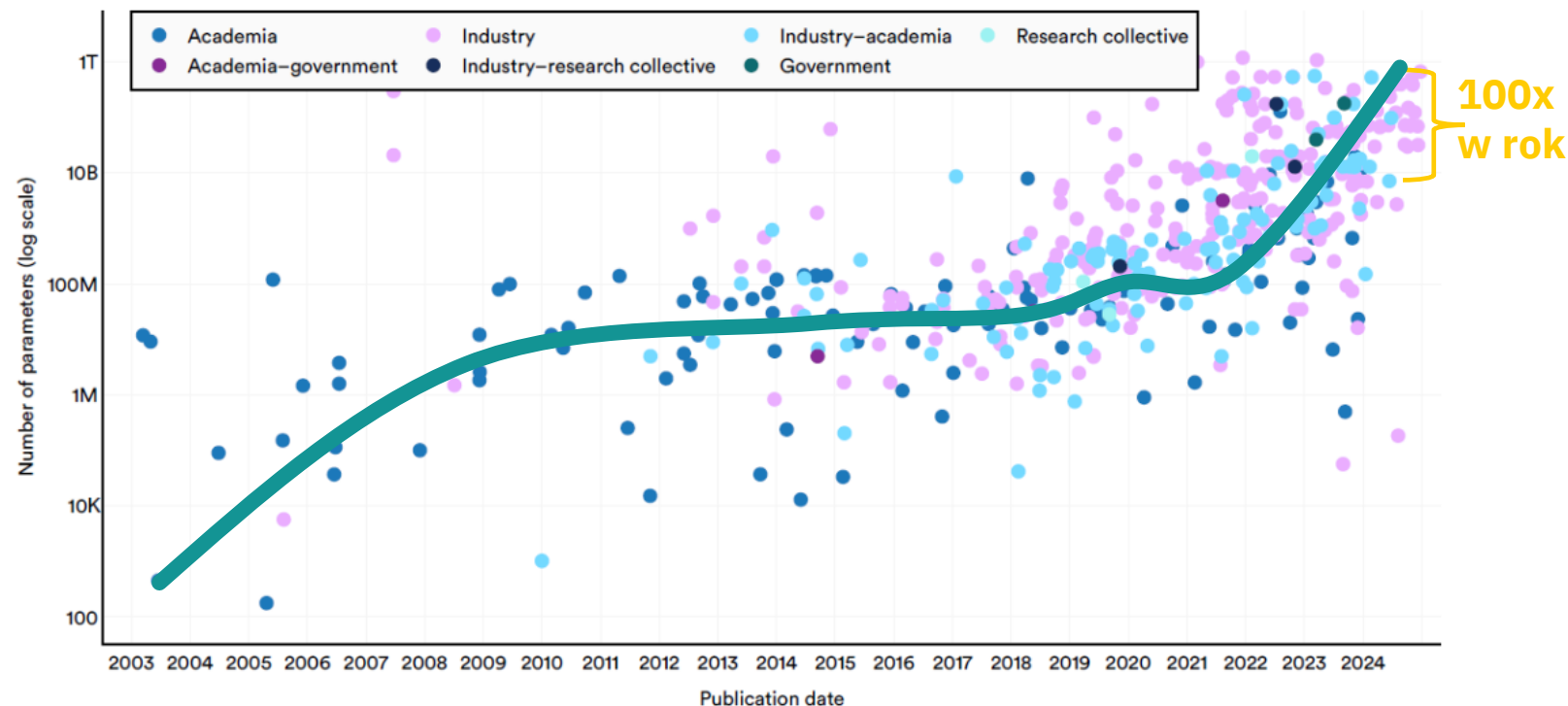
Number of parameters of notable AI models by sector, 2003–24
